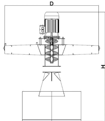
L- series surface aerator Front View
